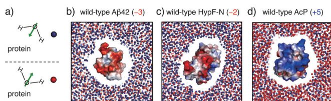
Figure 3. Long-range orientational distribution of the water surrounding the protein surface. The protein surfaces are colored according to the surface charge (blue for positively and red for negatively charged regions) and the water molecules, shown as spheres, are colored according to the direction of the dipole moment [blue indicates a dipole moment directed toward the protein and red indicates a dipole moment pointed away from the protein; see panel (a)]. Water molecules close ( < 8 \text{ \AA} ) to the protein surface, the orientation which depends on the local chemical details of the surface, are not shown. The orientational distribution of the water molecules at greater distances is determined primarily by the net charge of the protein. There are thus more “dipole-towards” (blue) water molecules around the negatively charged A \beta 42 (b) and HypF-N (c), whereas there are more “dipole-away” (red) water molecules around the positively charged AcP (d). These long-range “polarized” water molecules in turn discriminate between charged residues on the protein surface.
