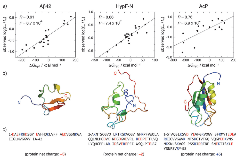
Figure 1. Correlation between experimental protein aggregation propensity and calculated protein hydrophobicity. a) Changes in the experimental aggregation propensity \log(f_{\text{mut}}/f_{\text{wt}}) upon mutation are plotted against the difference in the hydration free energy [\Delta G_{\text{hyd}} = G_{\text{hyd}}(\text{mut}) - G_{\text{hyd}}(\text{wt})] for the mutant and wild-type variants of Aβ42 (left-hand panels), HypF-N (middle panels), and AcP (right-hand panels). The Pearson correlation coefficient ( R ) and statistical significance ( P value) are also displayed. b) Snapshot structures generated by simulations for the intrinsically disordered Aβ42, the folding-incompetent HypF-N, and the folded form of AcP. Each structure is color-coded according to primary sequence, ranging from blue at the N terminus to red at the C terminus. c) Sequences for wild-type Aβ42, HypF-N, and AcP. Positively charged residues are indicated in blue, negatively charged residues in red, and neutral residues in black. The total net charge of each protein is also displayed.
